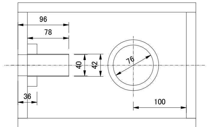
Section "EE"
