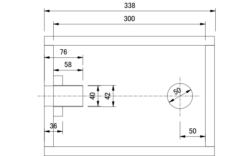
Section "CC"
